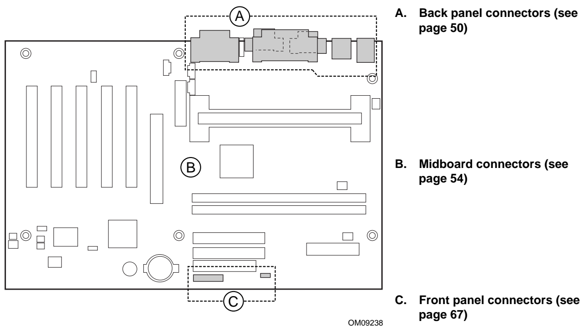
Figure 7. Connector Groups
