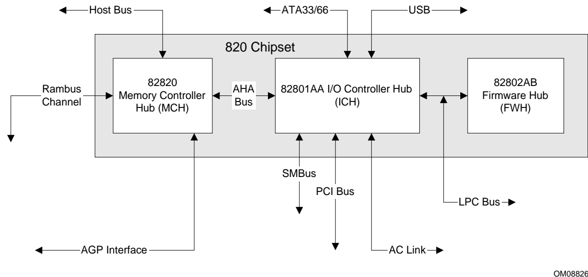
Figure 3. Intel 820 Chipset Block Diagram
