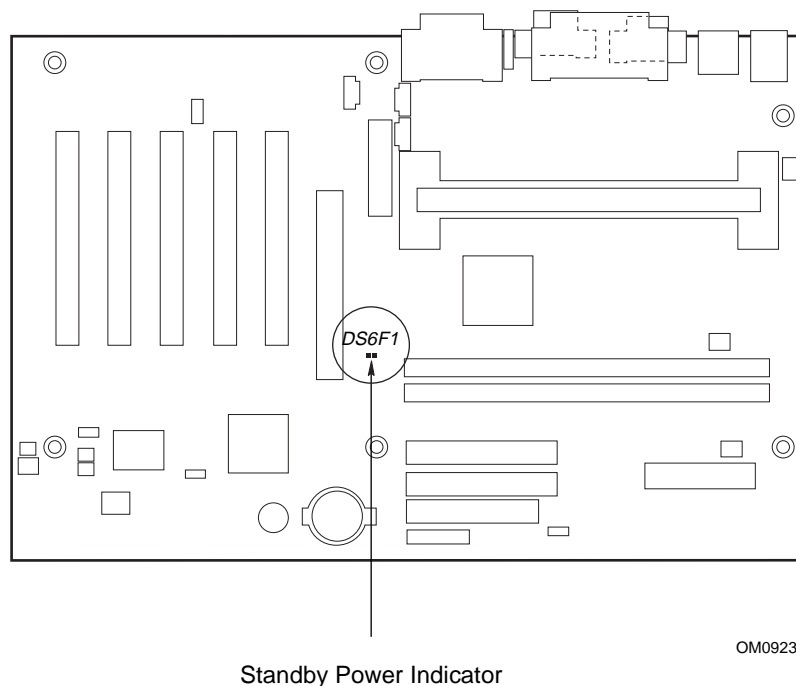
Figure 6. Location of Standby Power Indicator LED
