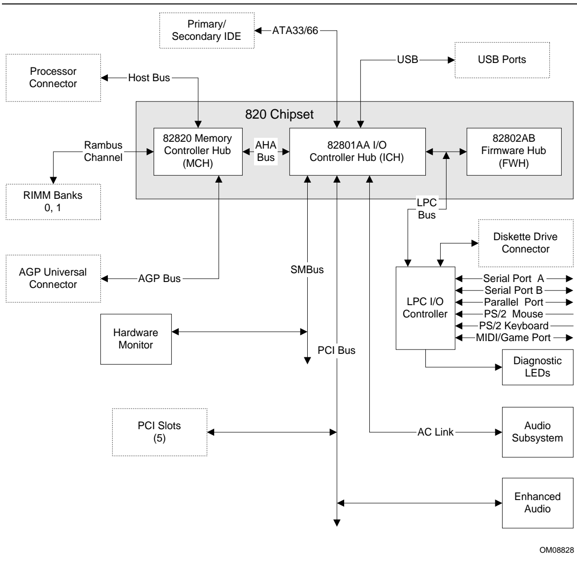
Figure 2. Block Diagram
