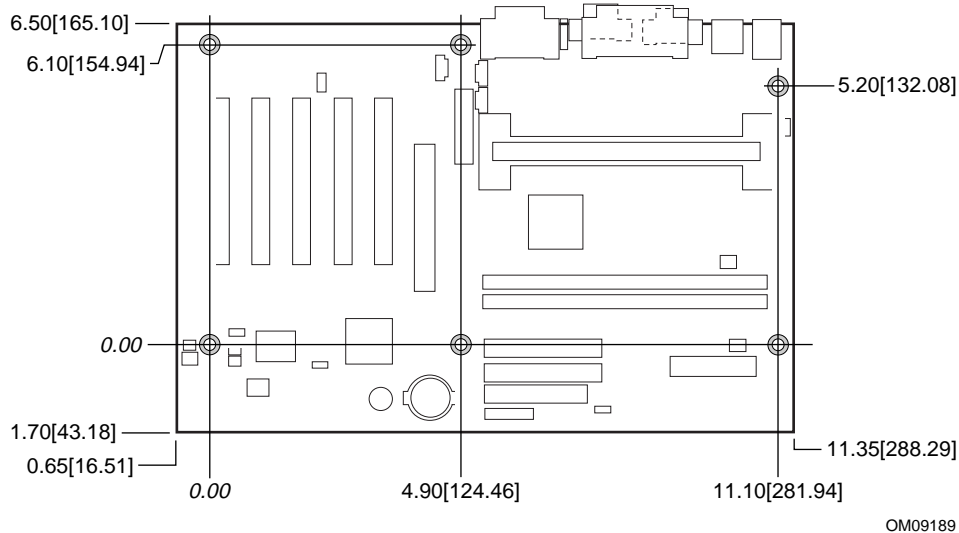
Figure 15. VC820 Board Dimensions
