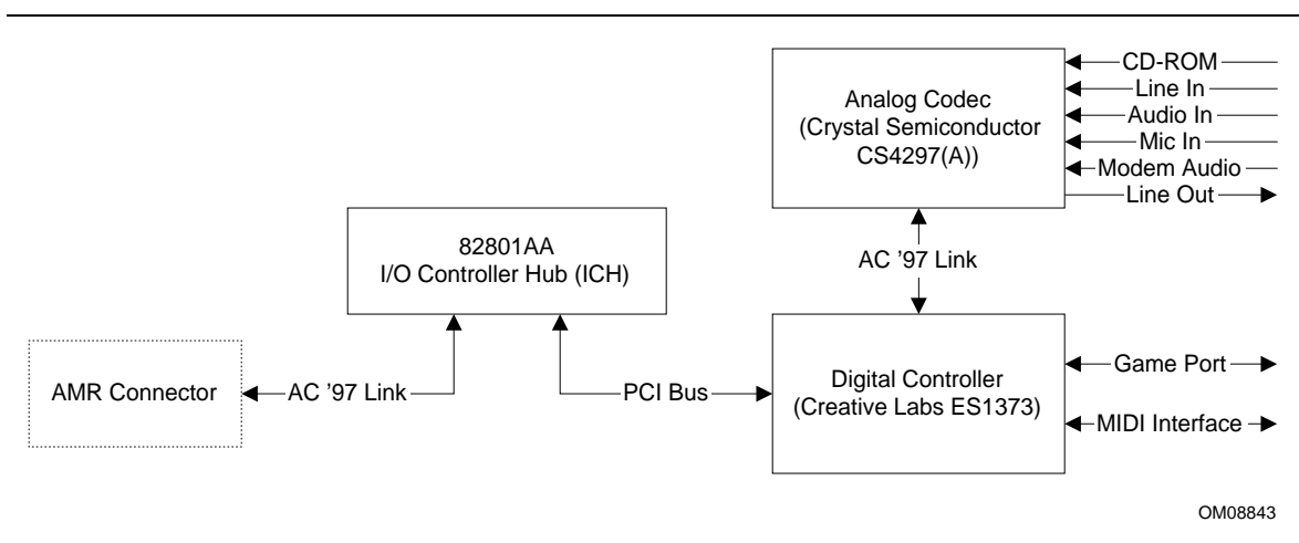
Figure 4. Block Diagram of AC '97 V 1.03 Compatible Audio Subsystem with Creative Labs ES1373 Controller and AMR Connector
