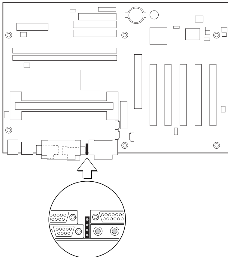
Figure 19. Enhanced Diagnostic LEDs
