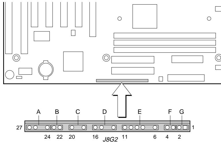
Figure 5. Front Panel I/O Connectors
