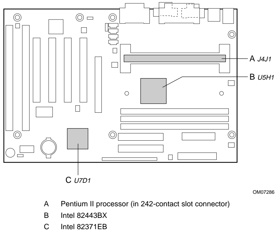
Figure 10. Thermally-Sensitive Components
