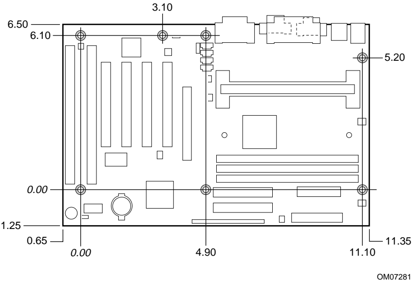
Figure 7. Motherboard Dimensions
